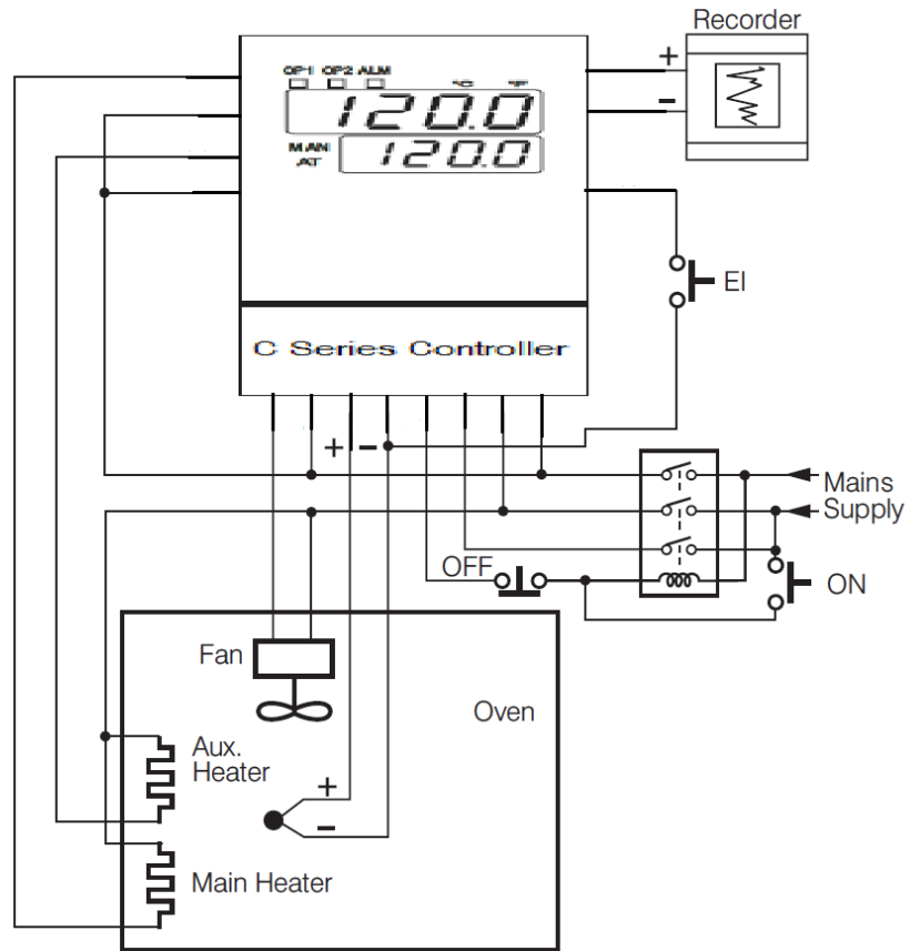
4-11 Heat Treatment Chamber
