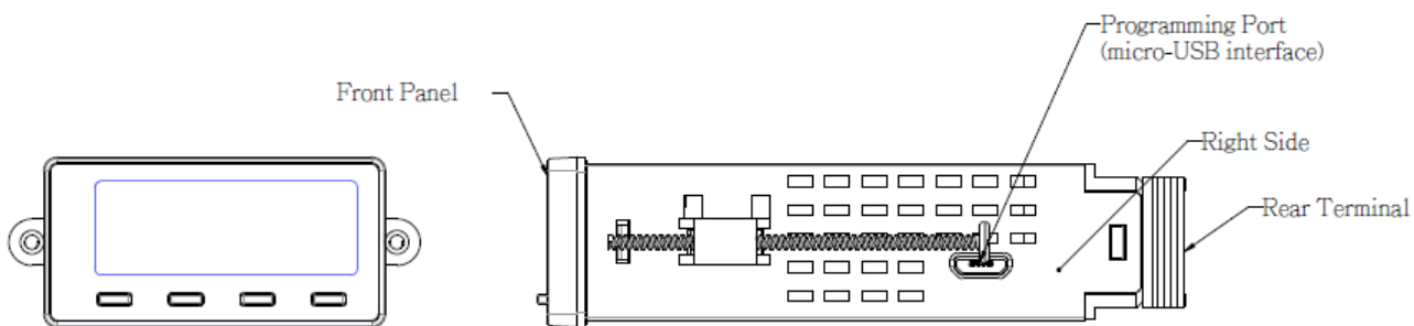
2-1 C22 Dimensions with clamp
