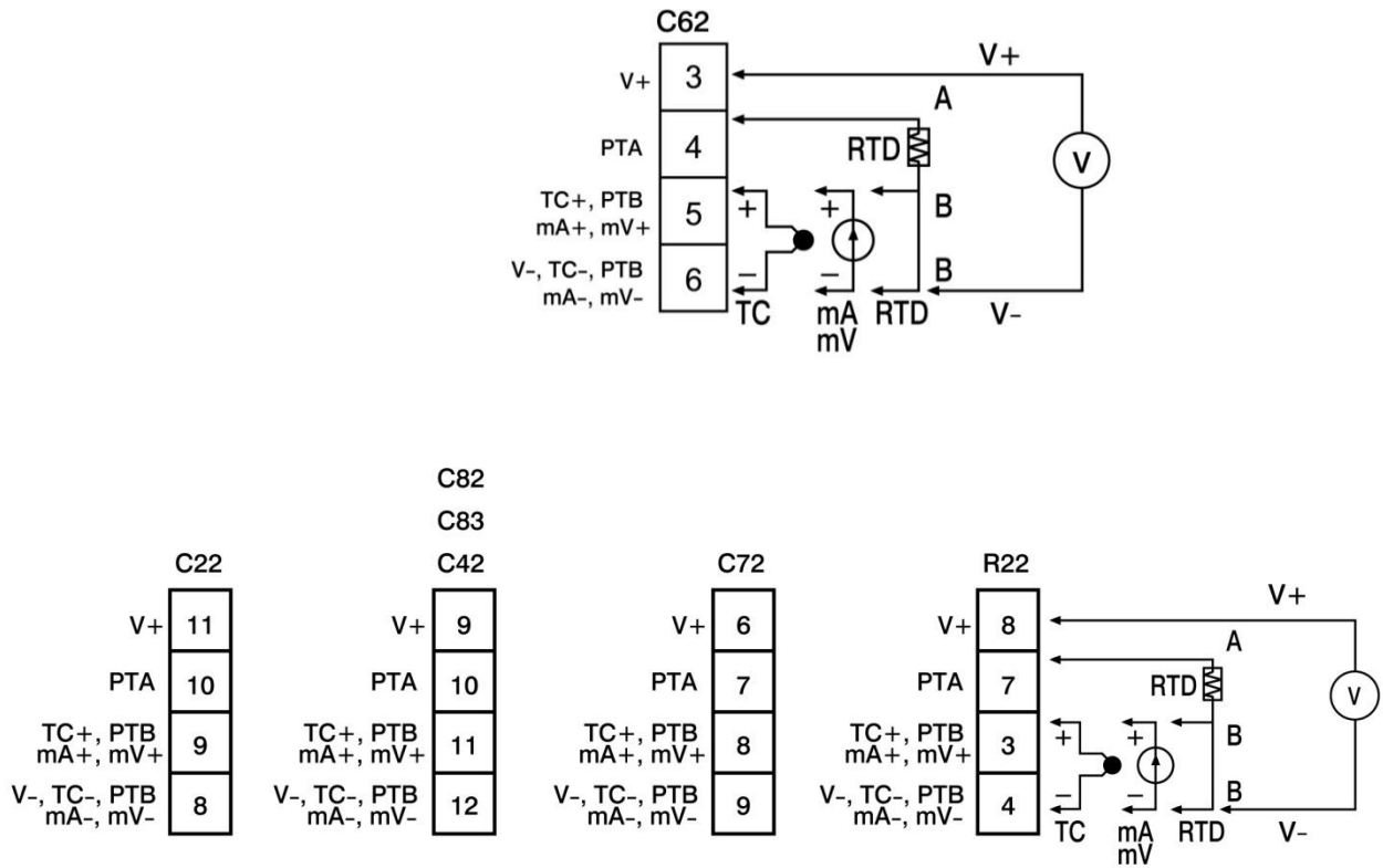
2-25 Sensor Input Wiring
