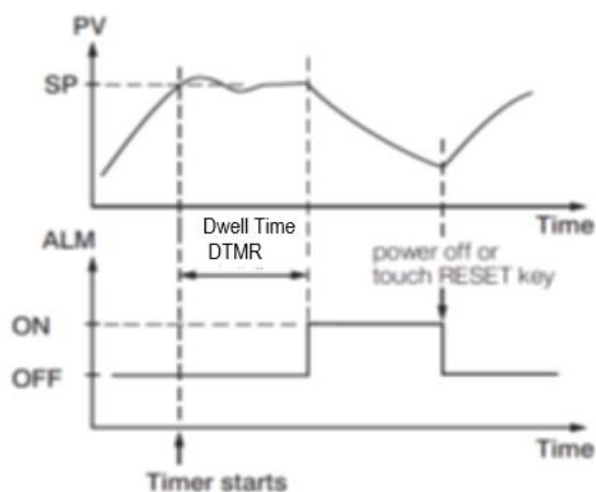
3-23 Dwell Timer
