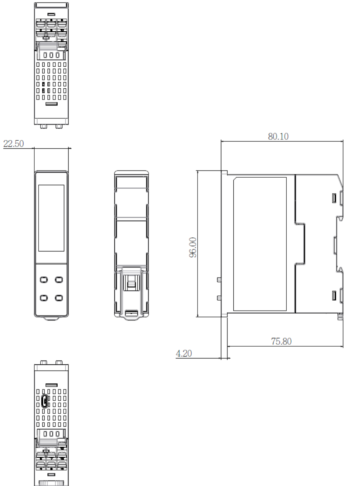
2-13 R22 Dimension
