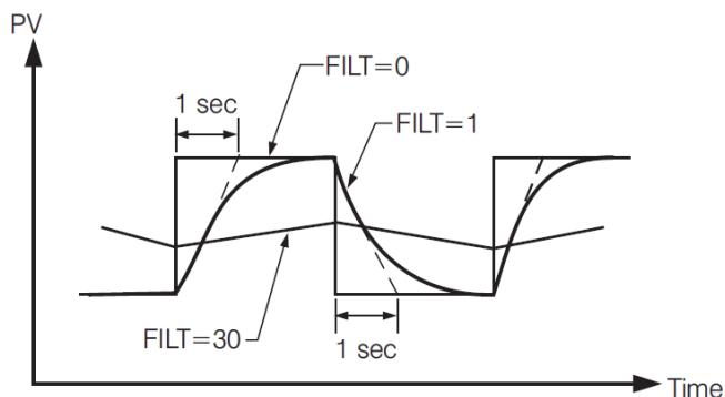
3-25 Filter Characteristics
