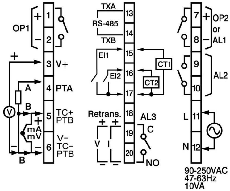
2-19 C62 Rear Terminal Connection
