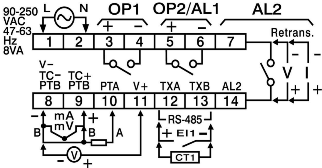
2-18 C22 Rear Terminal Connection
