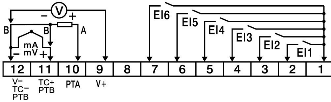
2-21 C83 Rear Terminal Connection
